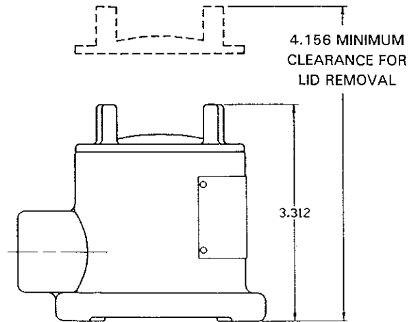
REMOTE TRANSDUCER
